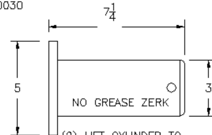
(2) LIFT CYLINDER TO LOWER PLOW ARM PART #4752-0031
